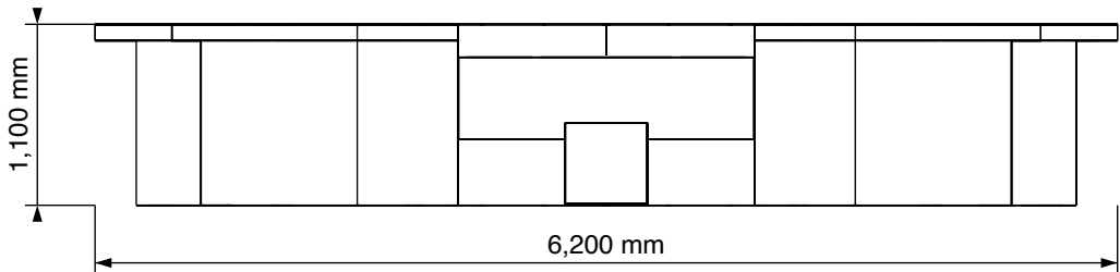
VISTA FRONTAL
